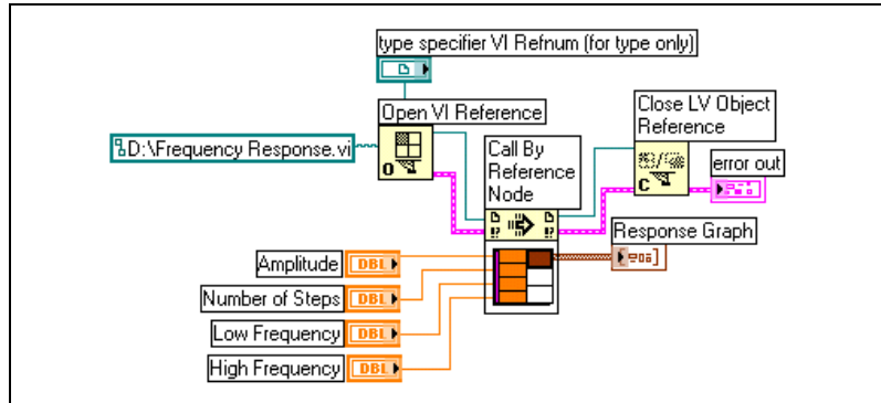
Figure 16-5. Using the Call By Reference Node
