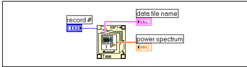
Figure 13-9. Retrieving Logged Data through SubVI Terminals
