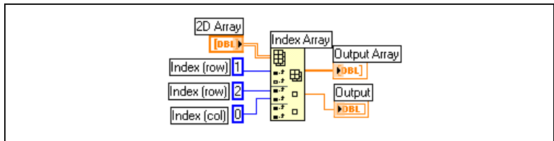
Figure 9-9. Indexing a 2D Array
