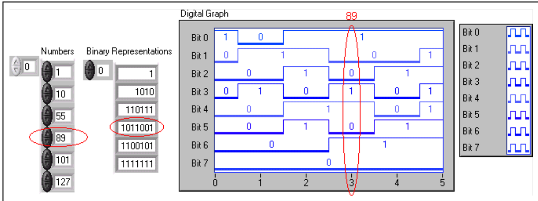
Figure 11-6. Graphing Integers Digitally
