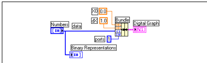
Figure 11-7. Using Bundle Function with Digital Graph
